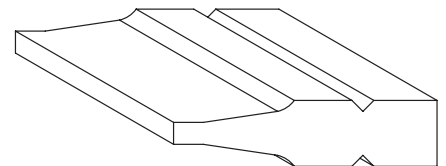
131 Vee Groove - 3/4" panel 1/4" w. x 1/8" d. vee groove
